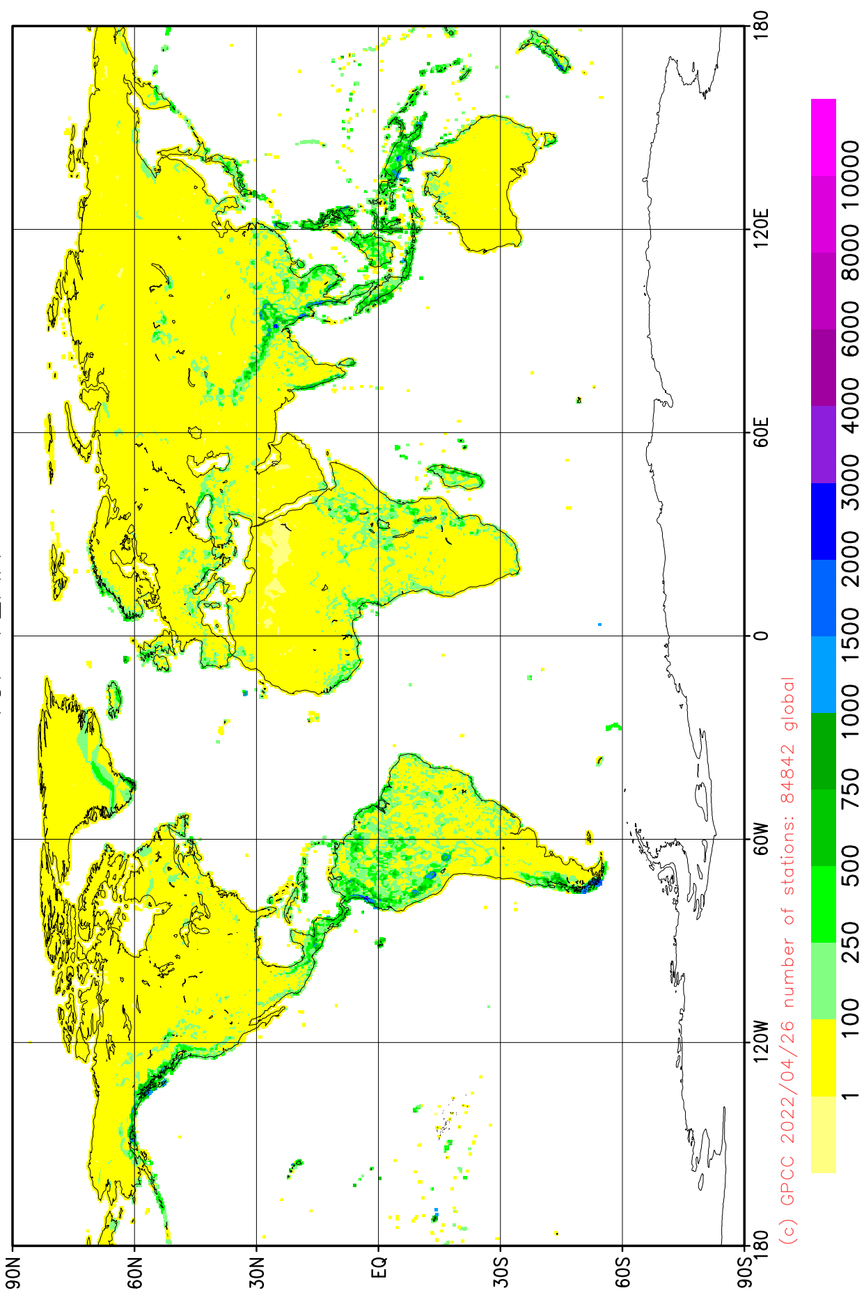
GPCC Precipitation Normals in mm/year (Version 2022) interpolation error per 0.25 degree grid for YEAR
